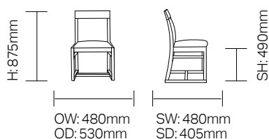
DCAV08 - Strengthened Side Chair with Braced Ski Leg
