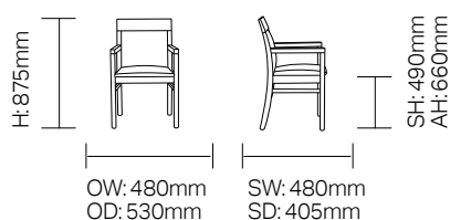
DCAV02M - Armchair; M-Spec
