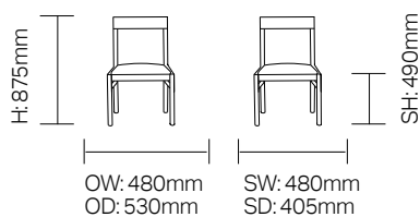
DCAV01M - Avenue Side Chair; M-Spec
