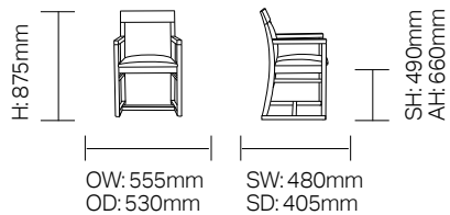
DCAV09 - Strengthened Armchair with Braced Ski Leg
