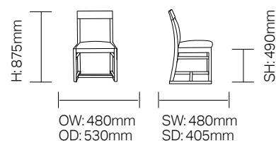
DCAV08M - Strengthened Side Chair with Braced Ski Leg; M-Spec
