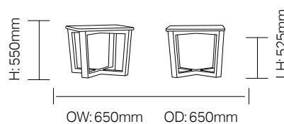
TCAR02X- Arcus 650sq Coffee Table X-Spec Weight: 19Kg
