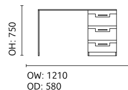
CAWE32 Dressing Table 3 Drawer Pedestal
