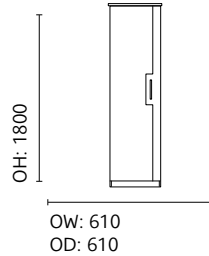
CAWE10 Single Wardrobe
