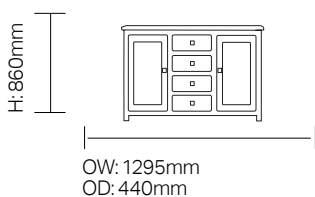
LCHP03 - Sideboard Unit LHF Door, Central 4 Drawers, RHF Door
