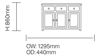
LCHP02 - Sideboard Unit 3 Drawers Over 3 Doors
